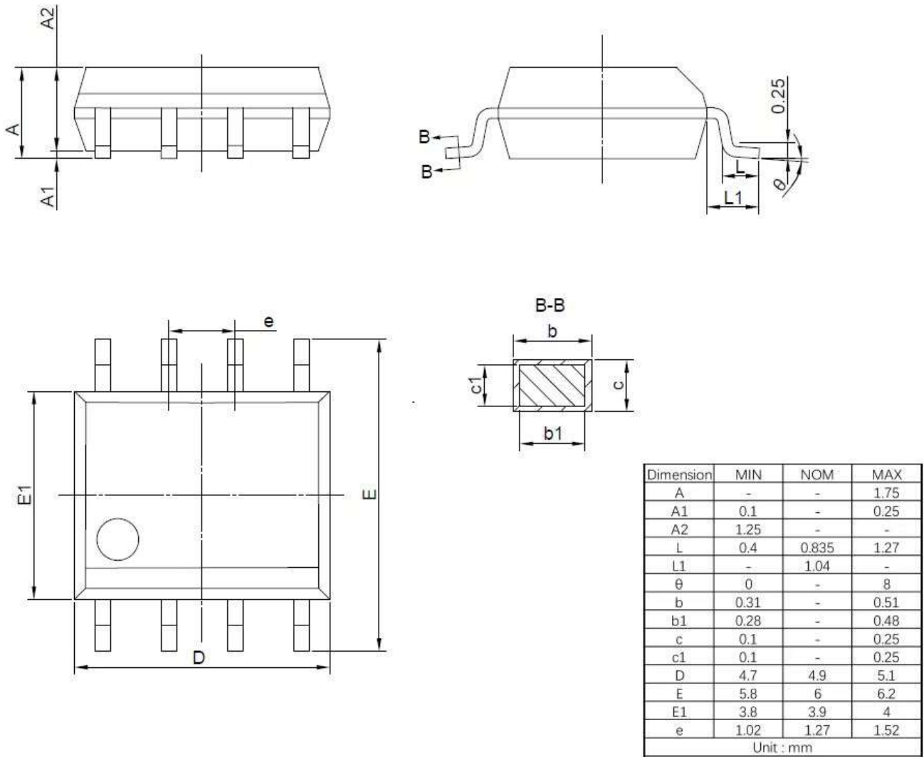
Figure 7. SOP8 Outline Dimensions
