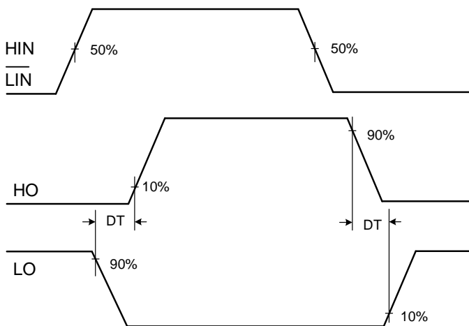
Figure 5. Dead Time Waveform
