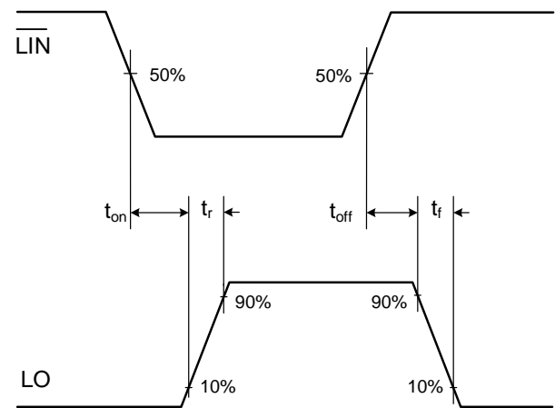
Figure 6. Low Side Switching Time Waveform
