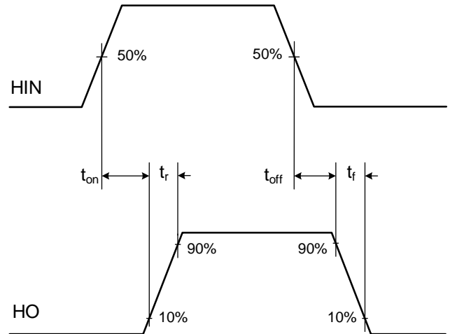
Figure 4. High Side Switching Time Waveform
