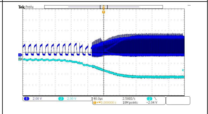
Figure 8. Vout1 Recovery from Short Line1: CP, Line2: Vout1
