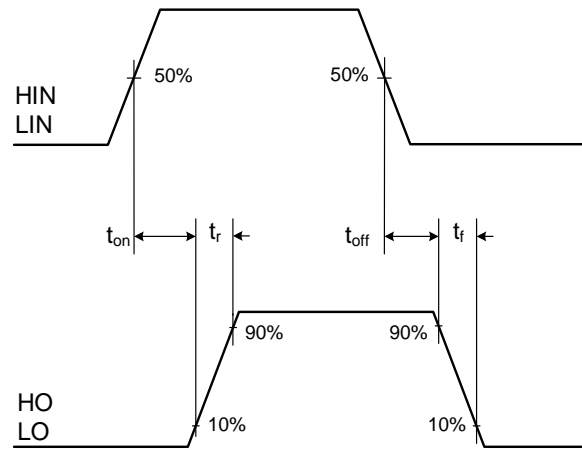
Figure 2. Switching Time Waveform
